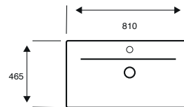
800MM MID BASIN
