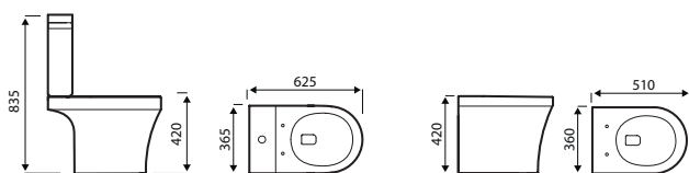
CLOSE COUPLED WC
